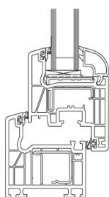
Profieldoorsnede CT70 Accent
